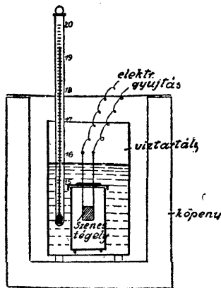
Kalorimeter
